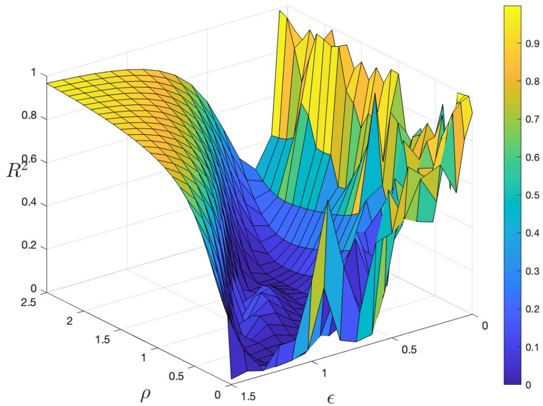
(b) R^2 from regressing \ln V_t on \frac{\alpha^r \psi}{1+\psi} \ln PY_t
