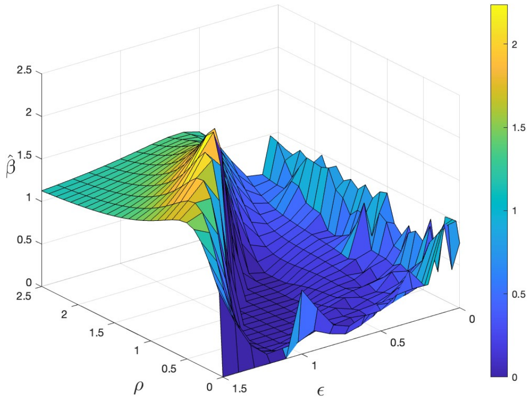
(a) \hat{\beta} from regressing \ln V_t on \frac{\alpha^r \psi}{1+\psi} \ln PY_t
