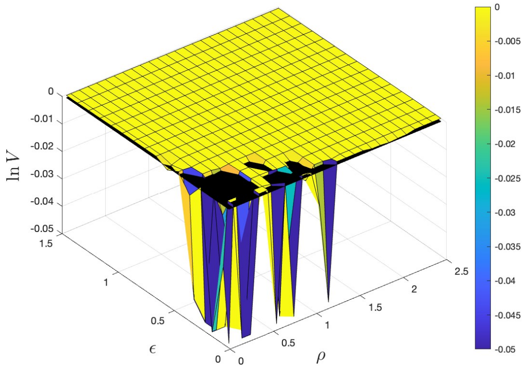
(b) Simulated \ln V_t vs. SHOTA implied approximation
