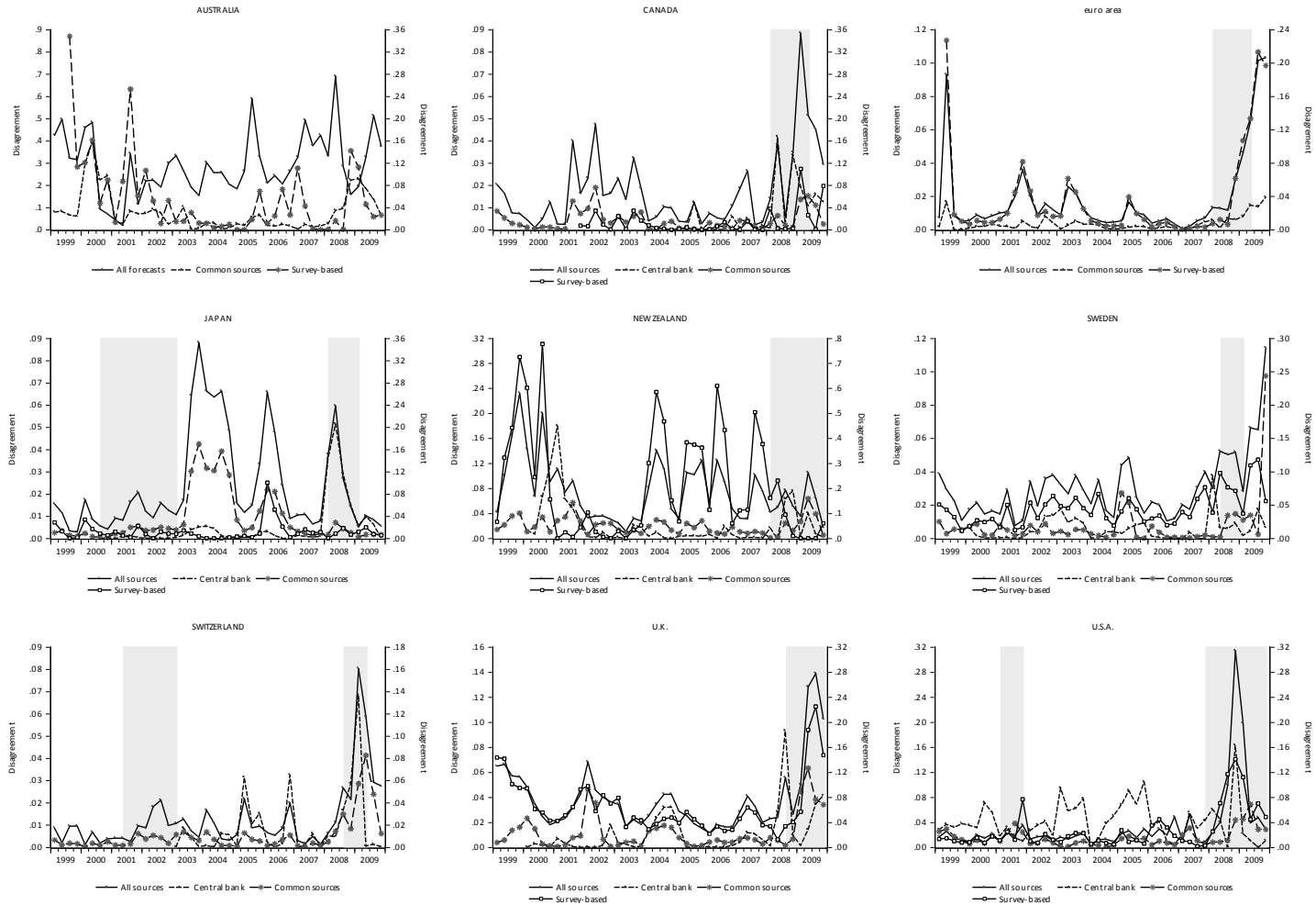
Figure 3 – Forecast Disagreement, 1999-2009
