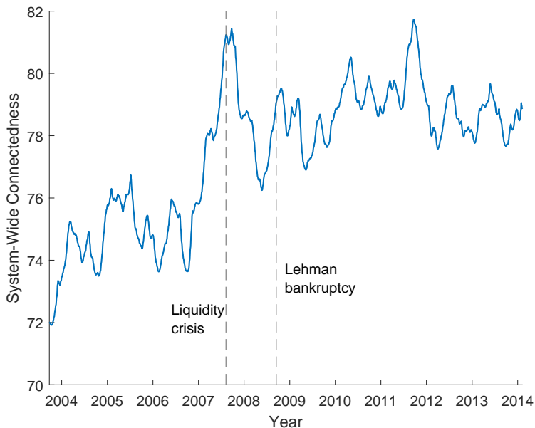
Figure 2: The dynamic system-wide connectedness measure from the VAR-SV.
