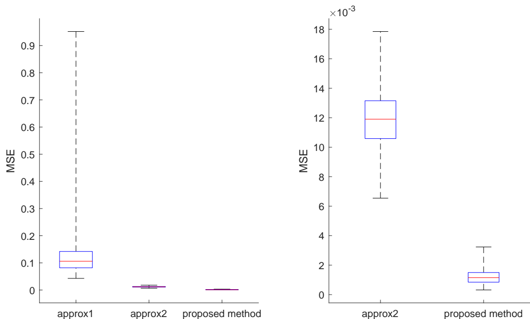
Figure 1: Boxplots of the mean squared errors for the three Gaussian approximations. Approx1 is the Gaussian distribution obtained by the \mathcal{N}(-1.27, \pi^2/4) approximation of the \log\text{-}\chi_1^2 distribution and approx2 is the Gaussian distribution based on a second-order Taylor approximation expanded around the mode of the target posterior distribution. The central mark indicates the median, whereas the bottom and top edges of the box indicate the 25-th and 75-th percentiles, respectively. The whiskers extend to the minimum and the maximum.
