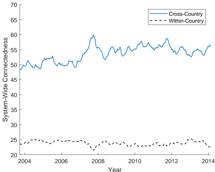
Figure 3: The decomposition of the dynamic system-wide connectedness measure from the VAR-SV into cross-country and within-country components.
