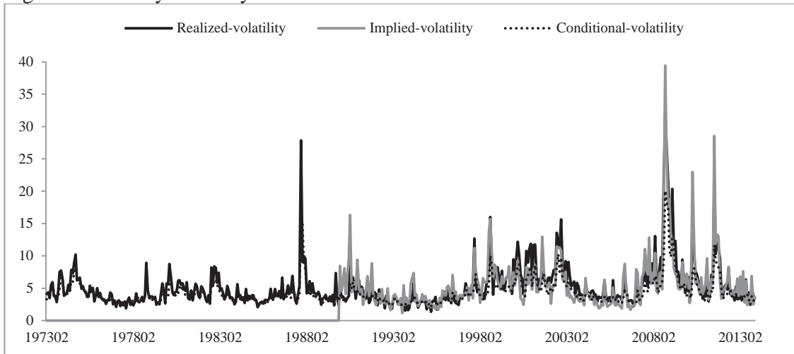
Figure 2: Monthly volatility of stock market return
