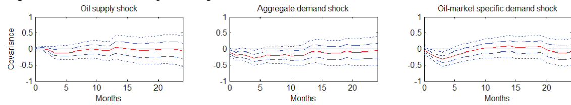
Figure 3B. Cumulative impulse responses of conditional-covariance
