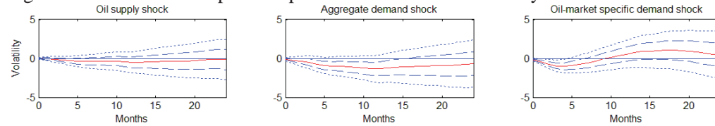
Figure 4B. Cumulative impulse responses of conditional-volatility
