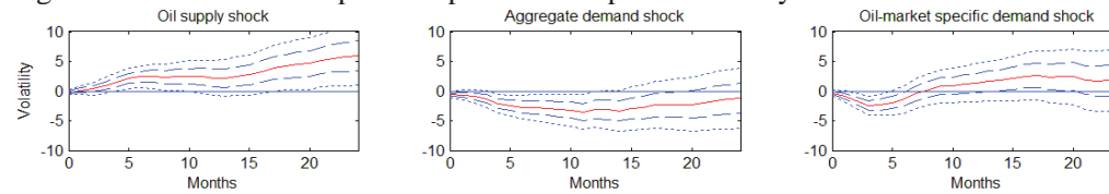
Figure 4C. Cumulative impulse responses of implied-volatility
