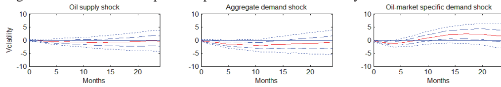
Figure 4A. Cumulative impulse responses of realized-volatility
