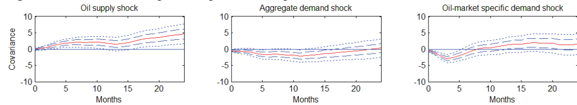
Figure 3C. Cumulative impulse responses of implied-covariance
