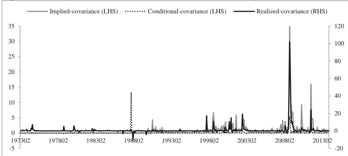
Figure 1: Monthly covariance of stock market return and volatility
