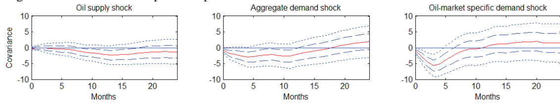
Figure 3A. Cumulative impulse responses of realized-covariance
