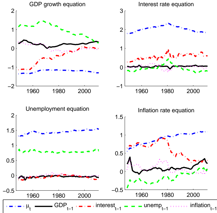
Figure 1: Evolution of the VAR coefficients \beta_t in the time-varying parameter VAR model.
