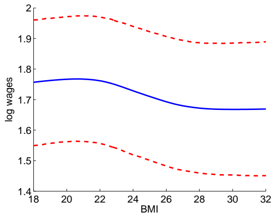
Figure 2: Posterior means of the function f(\cdot) with the prior mean \mathbb{E}\tau = 5 \times 10^{-6} (solid line) and the corresponding 90% credible intervals (dotted lines).
