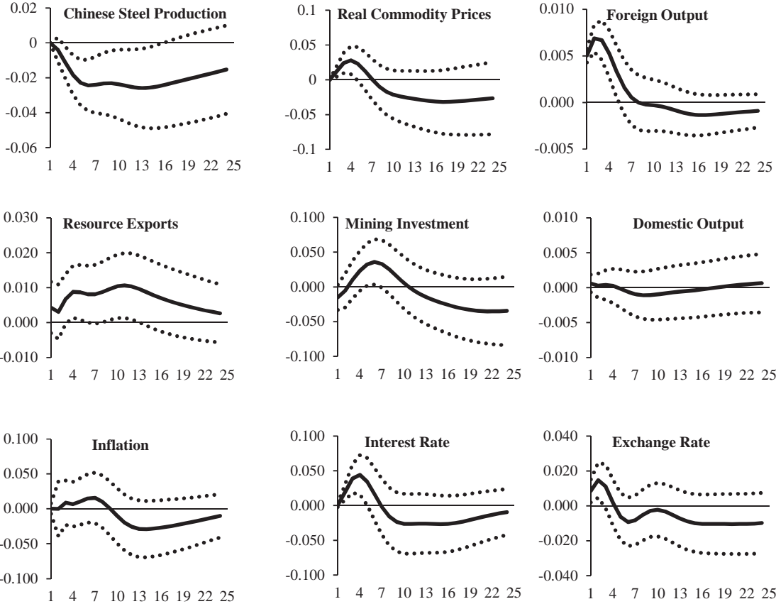
Figure 6: Impulse responses to shock to foreign output
